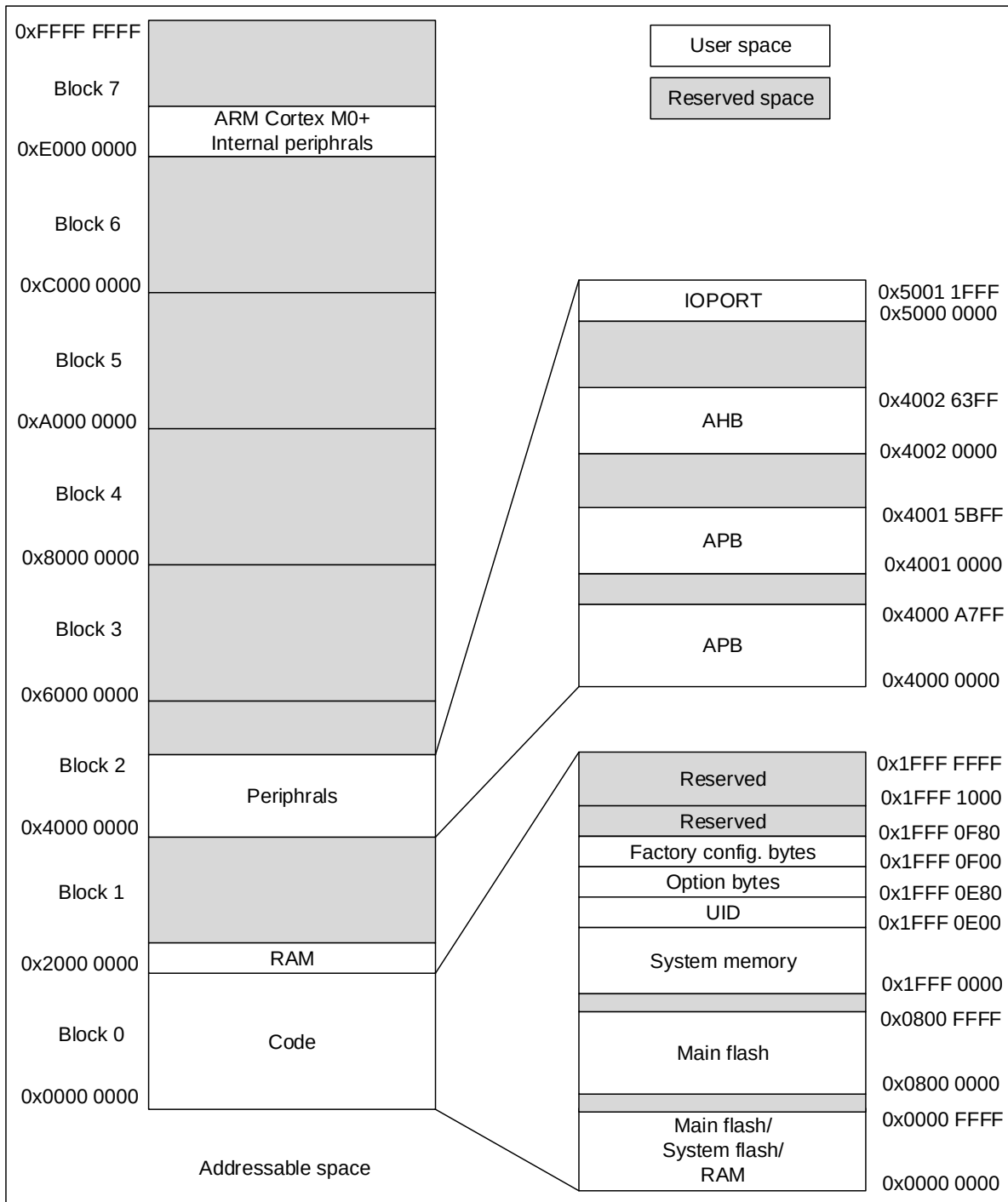
Figure 4-1 Memory map
