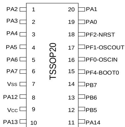
Figure 3-13 TSSOP20 Pinout2 PY32F030F2xPx / PY32F030F2xPx-E (Top view)
